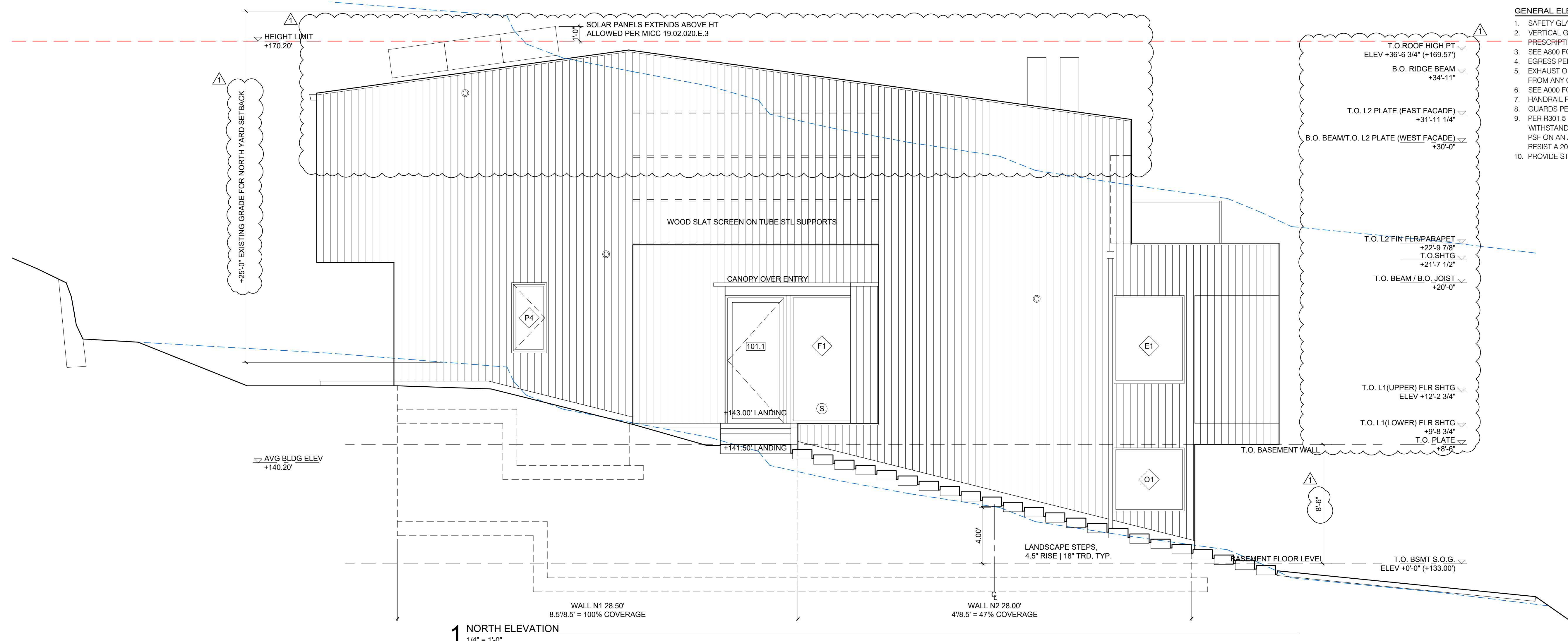
1 NORTH ELEVATION 1/4" = 1'-0"
