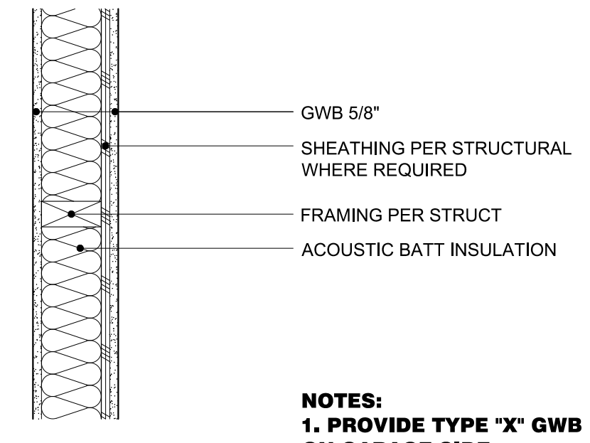
P1 PARTITION - TYPICAL INTERIOR 1 1/2"=1'-0"
