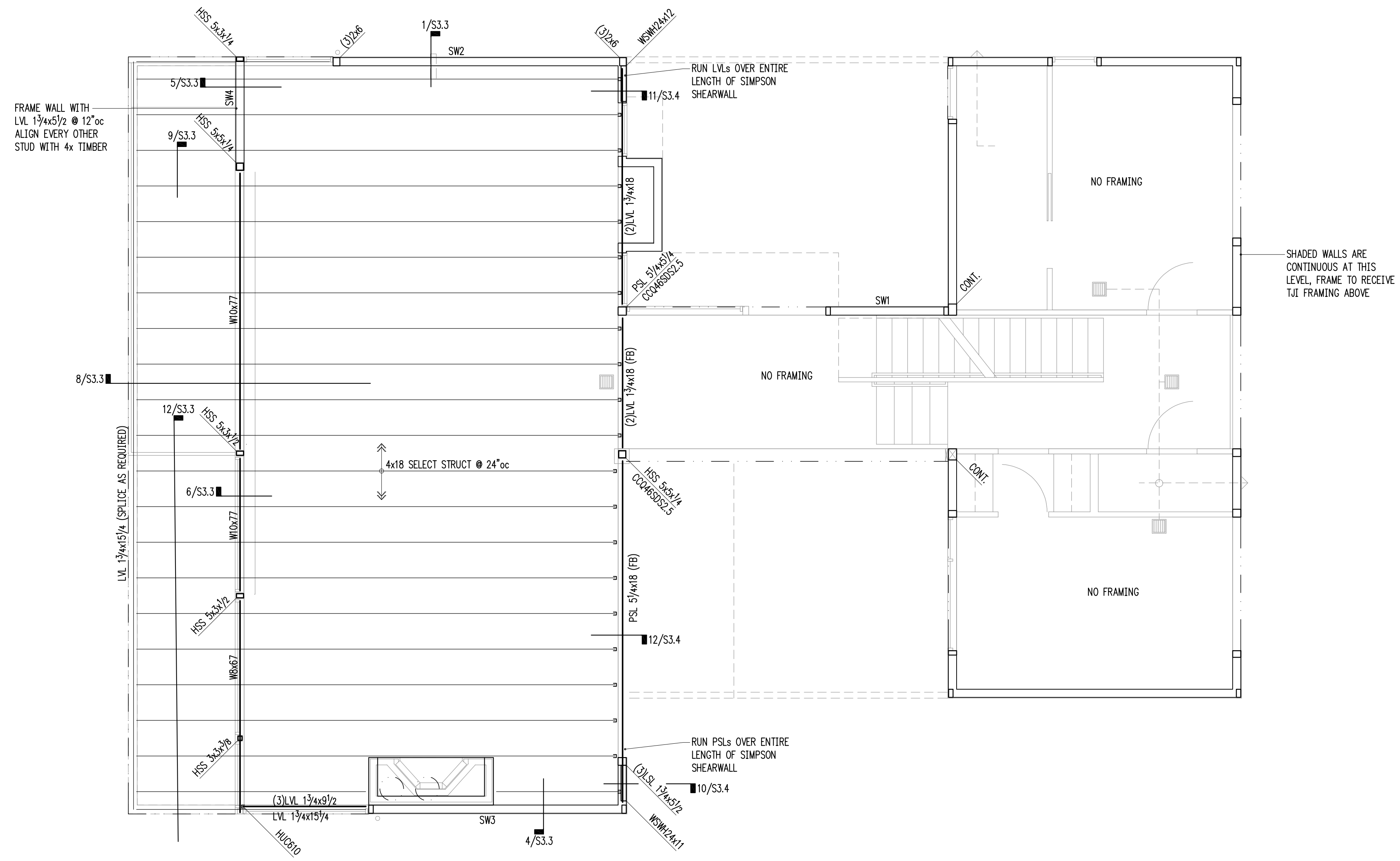
1 MAIN FLOOR CEILING FRAMING PLAN (MAIN FLOOR WALLS) S2.2 scale: 1/4" = 1'-0"
