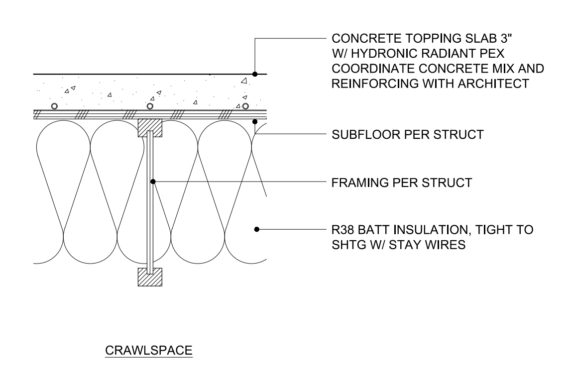
F3 FLOOR - TYPICAL OVER CRAWL SPACE 1 1/2"=1'-0"
