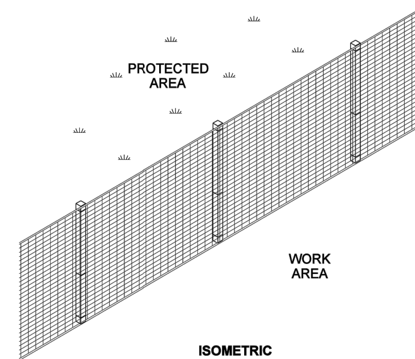
ISOMETRIC
