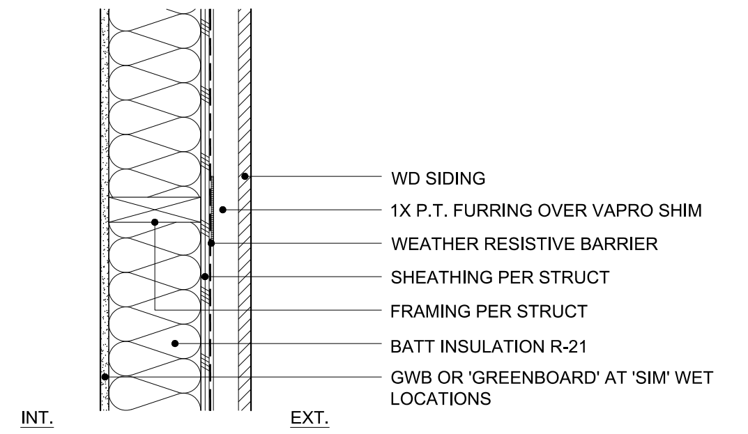
W1 WALL - TYPICAL EXTERIOR 1 1/2"=1'-0"
