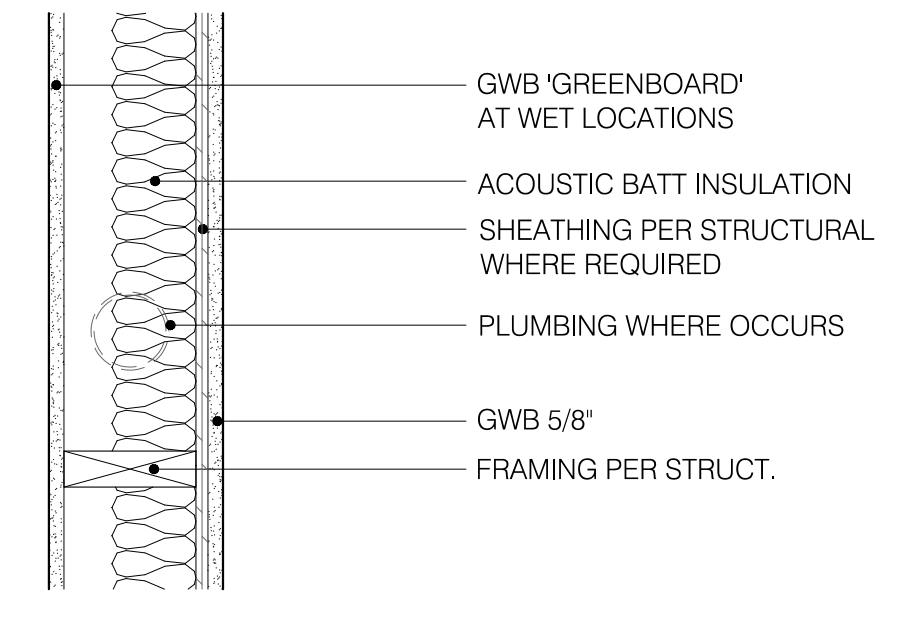
P2 PARTITION - TYPICAL PLUMBING 1 1/2"=1'-0"
