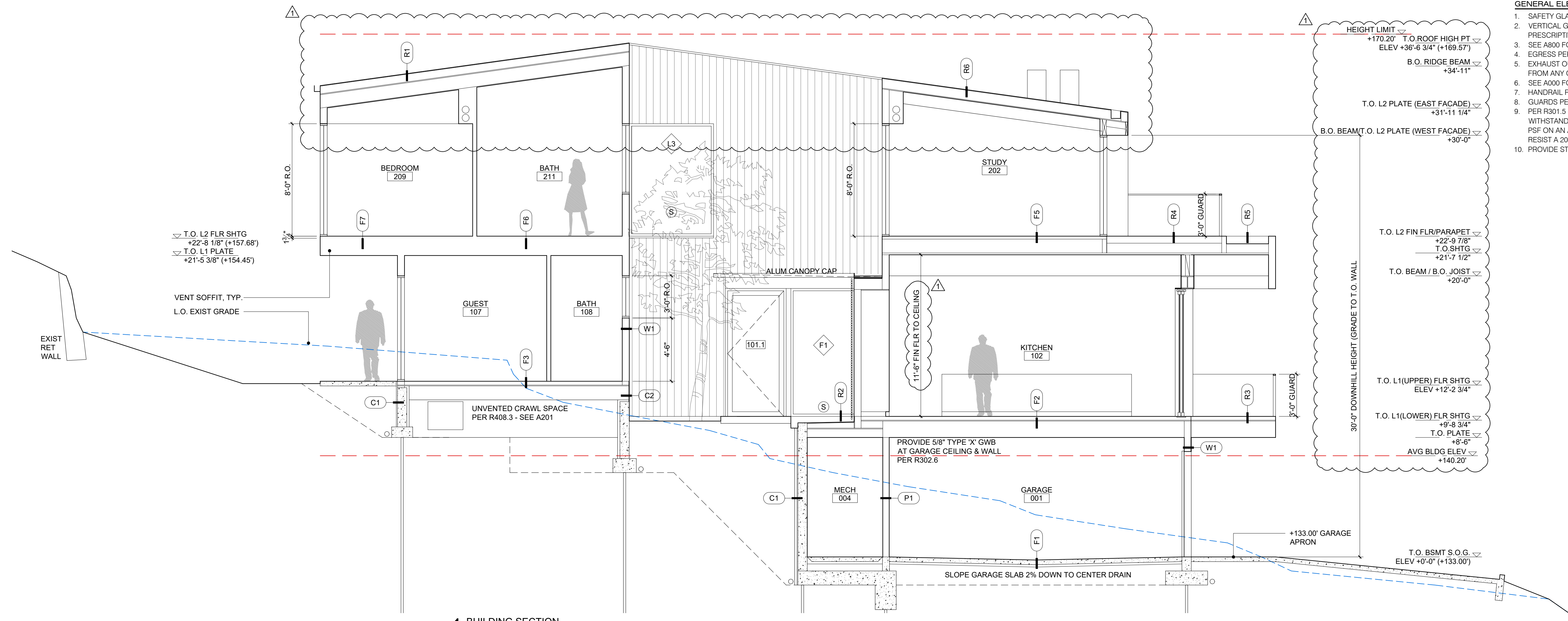
1 BUILDING SECTION 1/4" = 1'-0"
