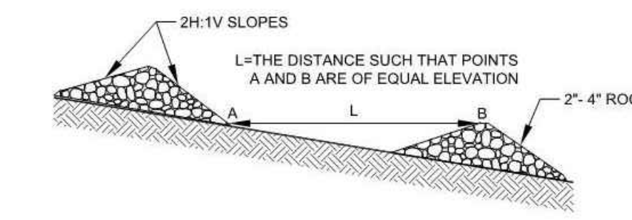
CHECK DAM SPACING
