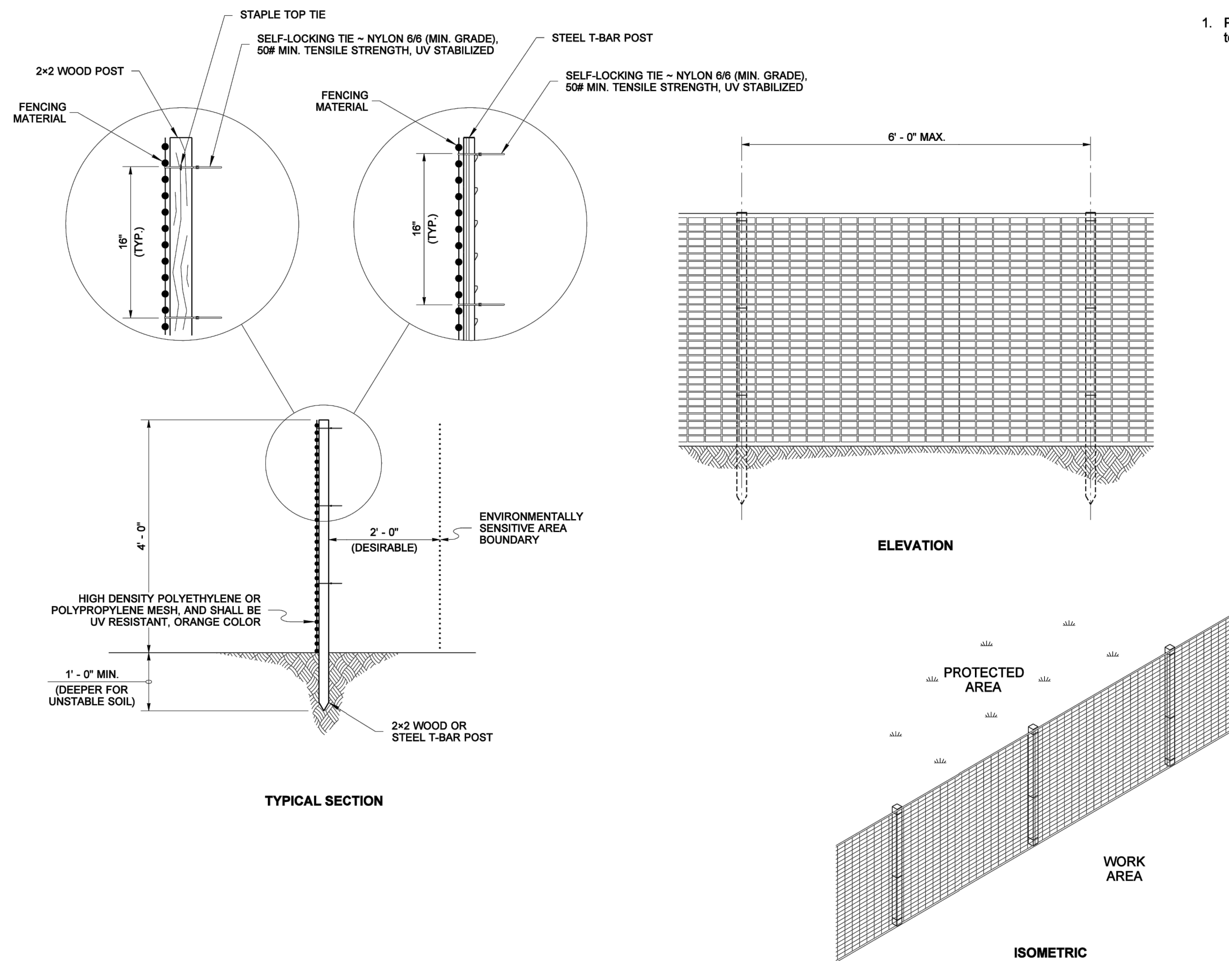
ISOMETRIC
