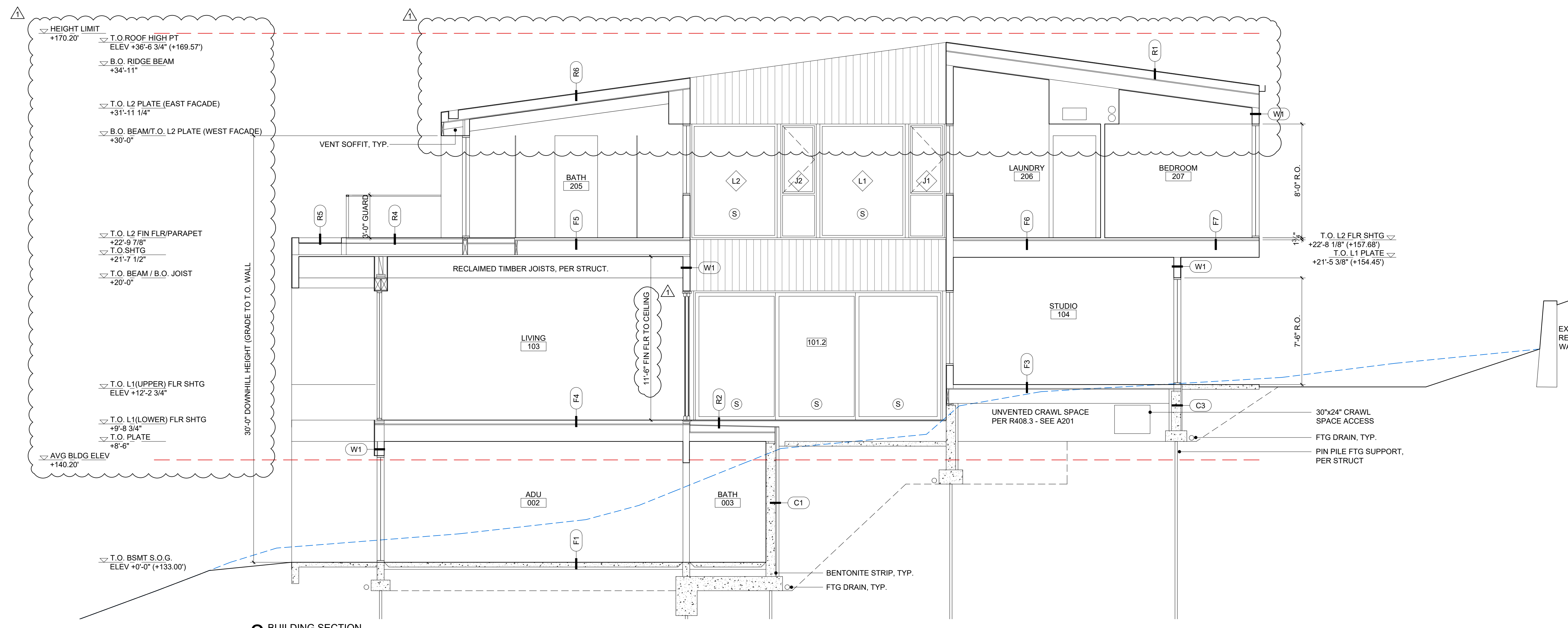
2 BUILDING SECTION 1/4" = 1'-0"
