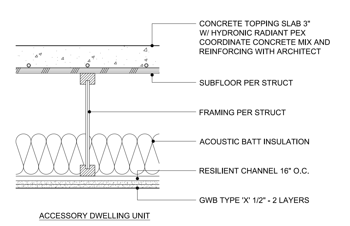
F4 FLOOR - LEVEL 1 OVER ADU 1 1/2"=1'-0"
