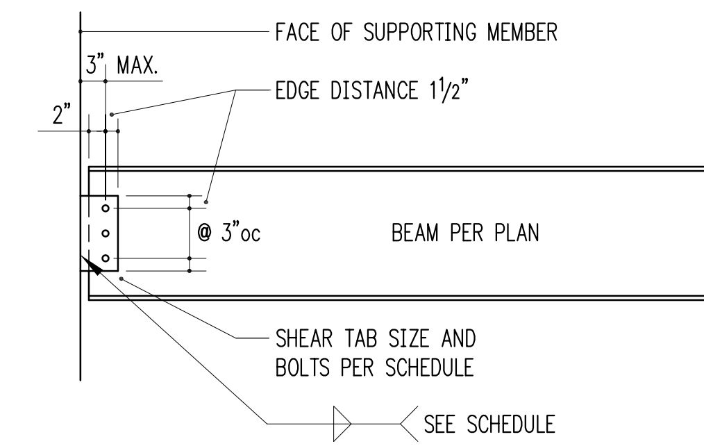
TYPICAL SHEAR TAB CONNECTION
