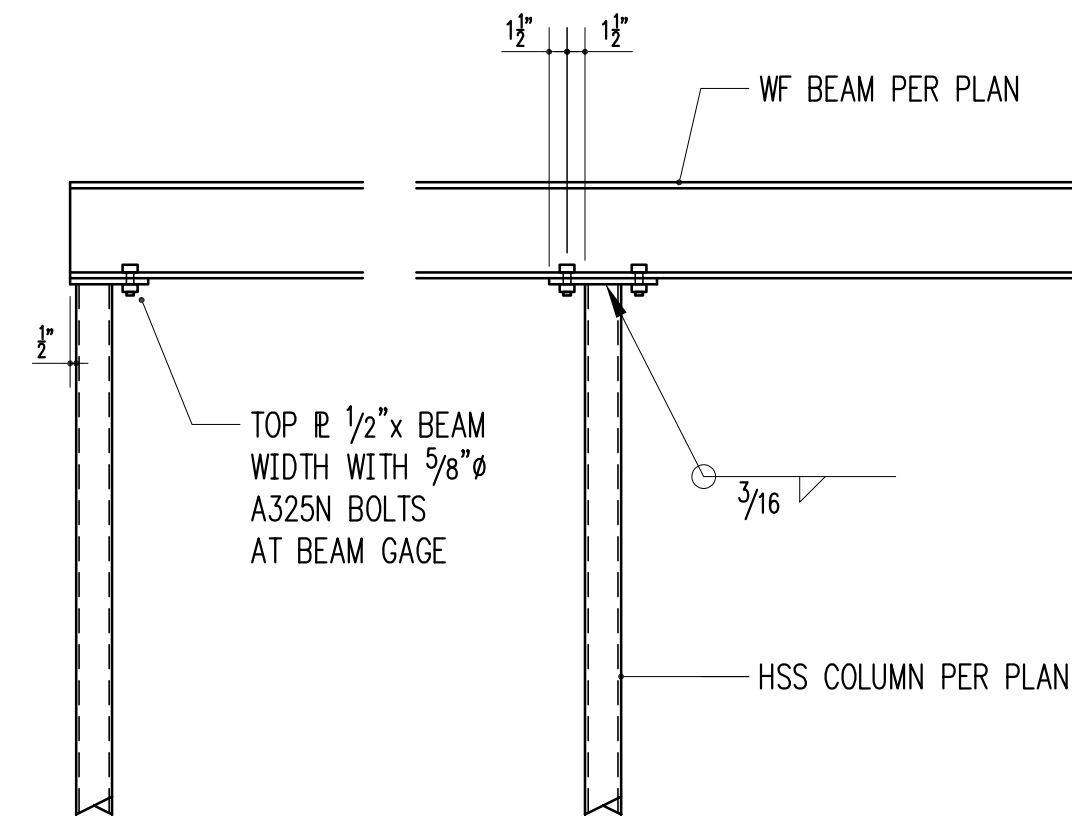
WF BEAM BEARING ON HSS COLUMN
