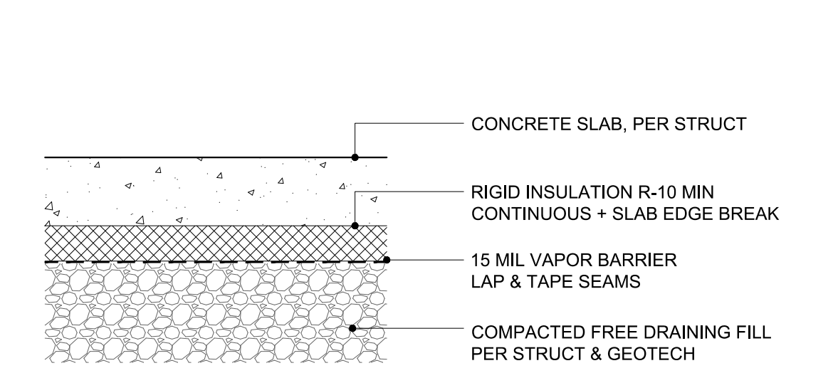
F6 FLOOR - TYPICAL LEVEL 2 1 1/2"=1'-0"
