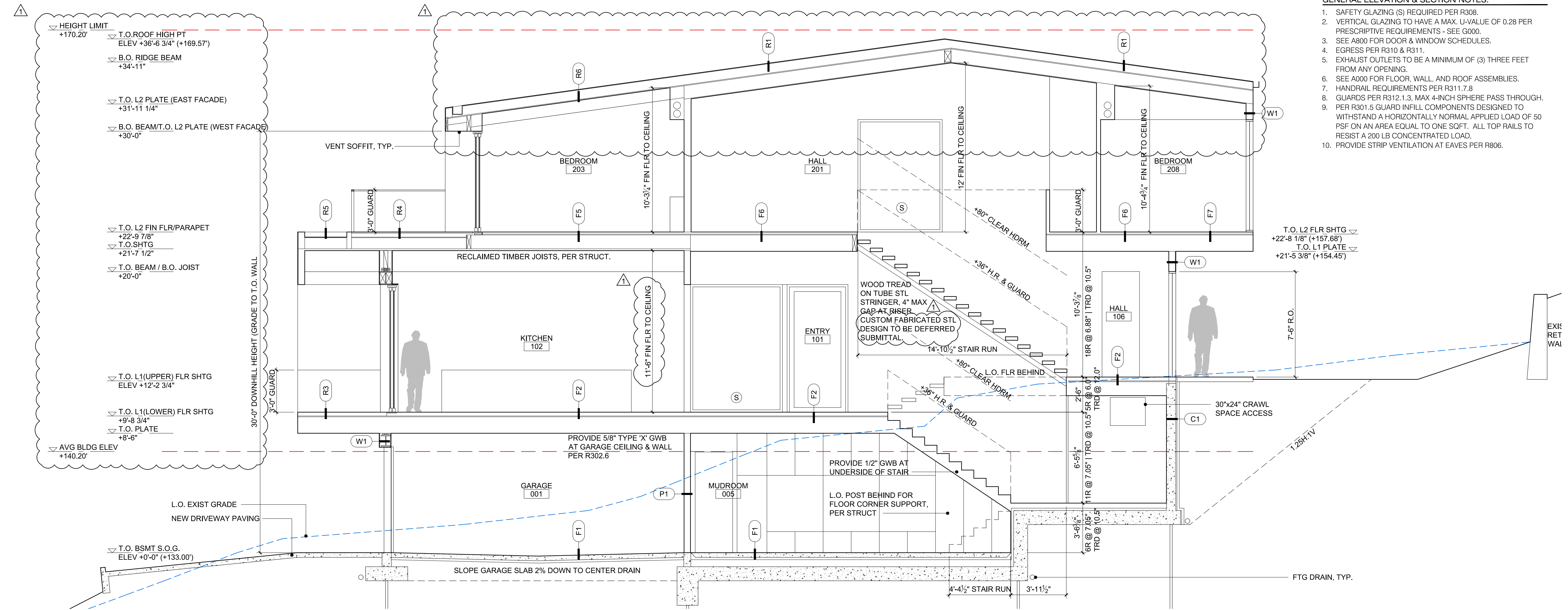
1 BUILDING SECTION 1/4" = 1'-0"
