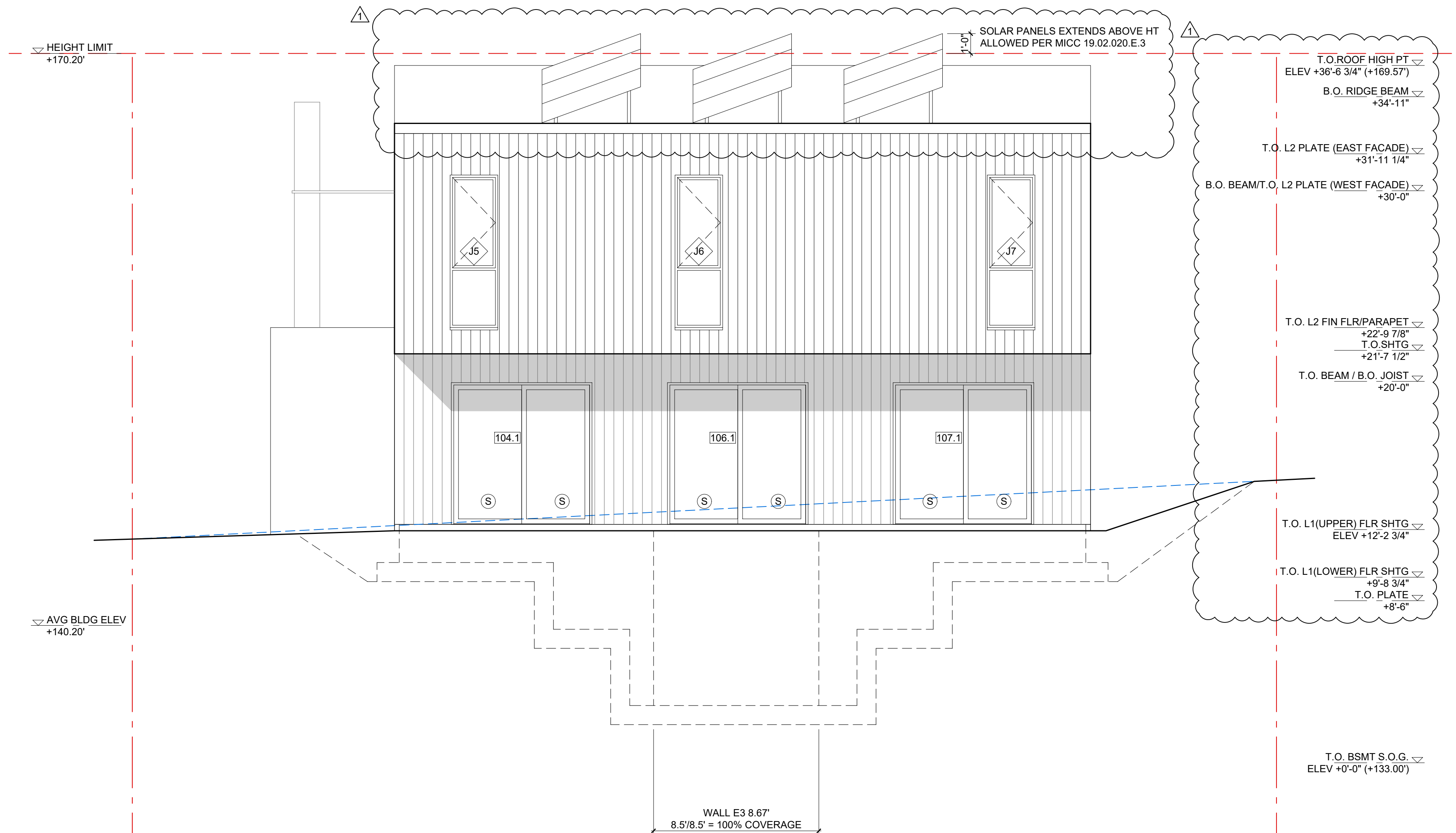
2 EAST ELEVATION 1/4" = 1'-0"
