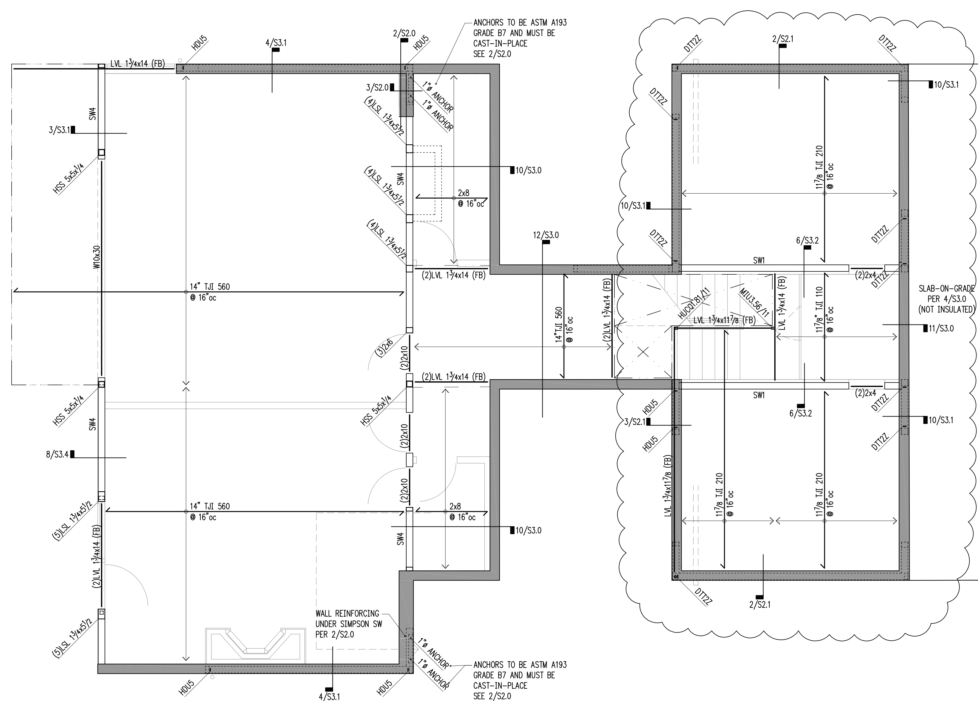
1 MAIN FLOOR FRAMING (BASEMENT WALLS) & UPPER FOUNDATION PLAN scale: 1/4" = 1'-0"
