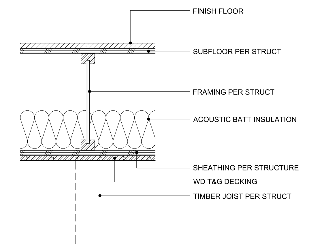
F5 FLOOR - TYPICAL LEVEL 2 1 1/2"=1'-0"
