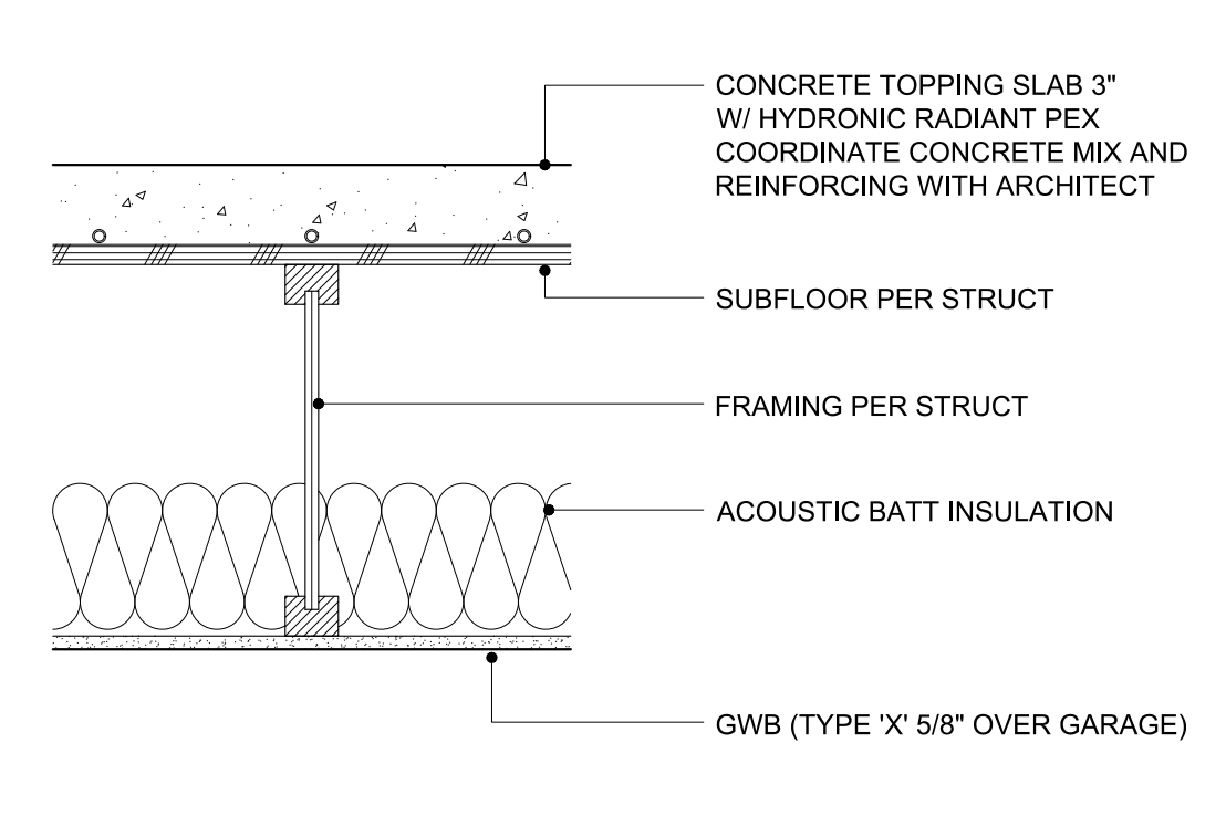
F2 FLOOR - TYPICAL LEVEL 1 1 1/2"=1'-0"
