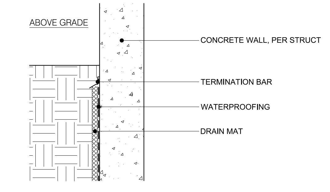
C3 WALL - CRAWL SPACE 1 1/2"=1'-0"
